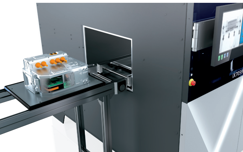
Special transport concept for handling assemblies on workpiece carriers or in solder frames
